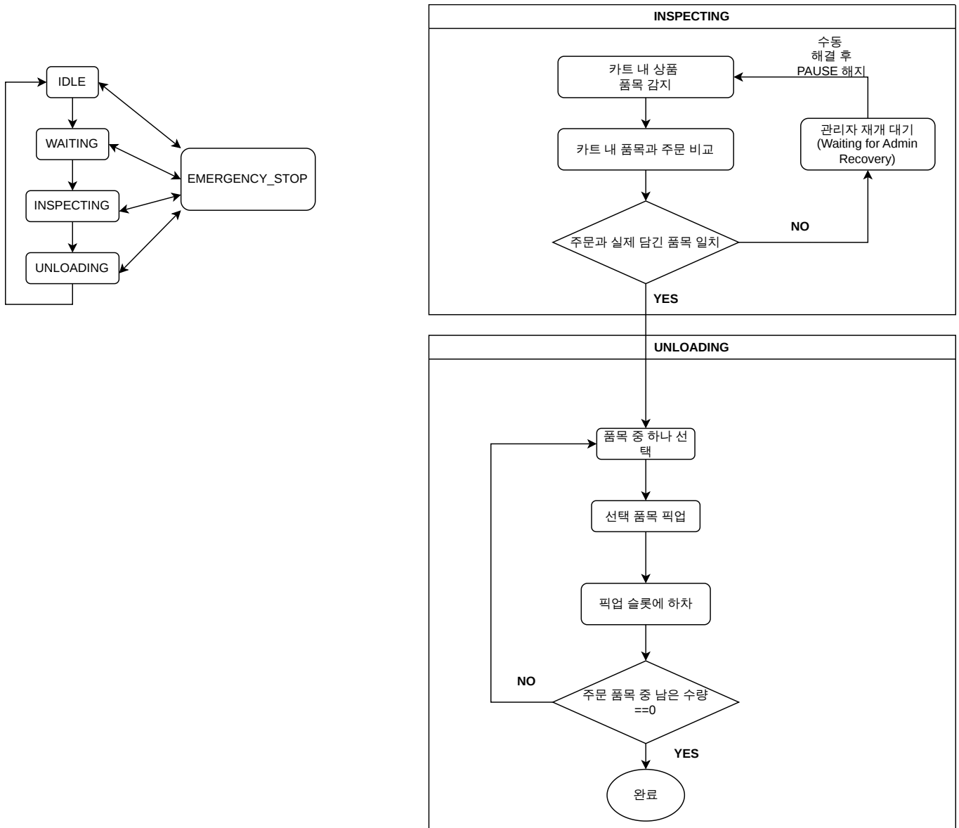
Inspection Cobot State Diagram (Inspection Cobot Status 중심)
